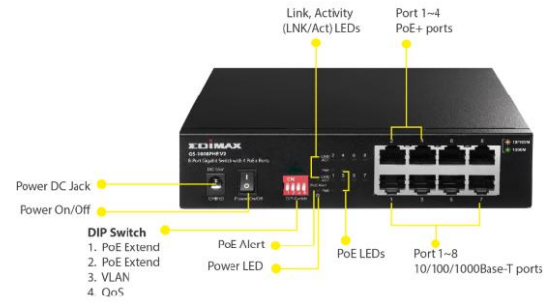
Front Panel
