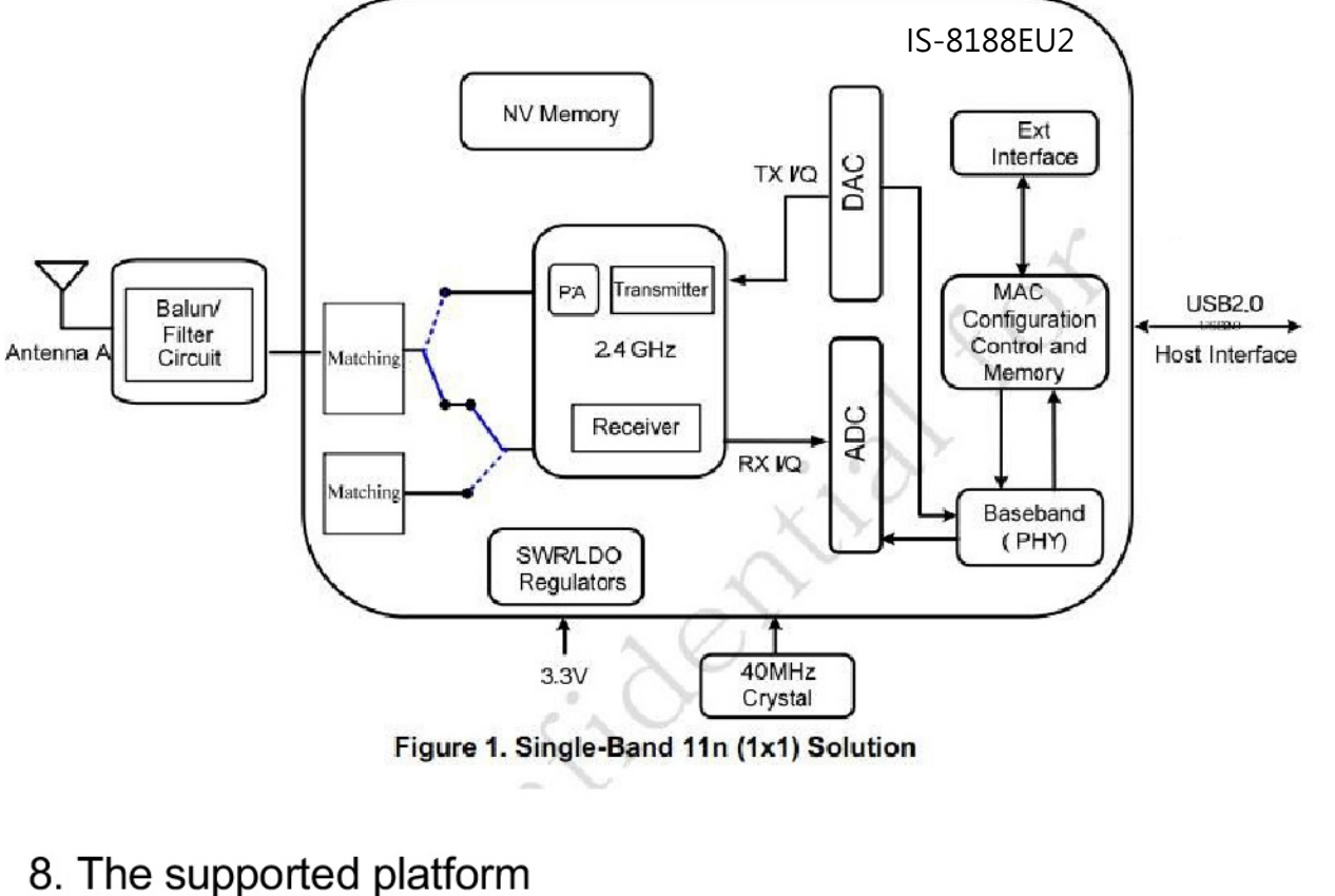
Figure 1. Single-Band 11n (1x1) Solution
